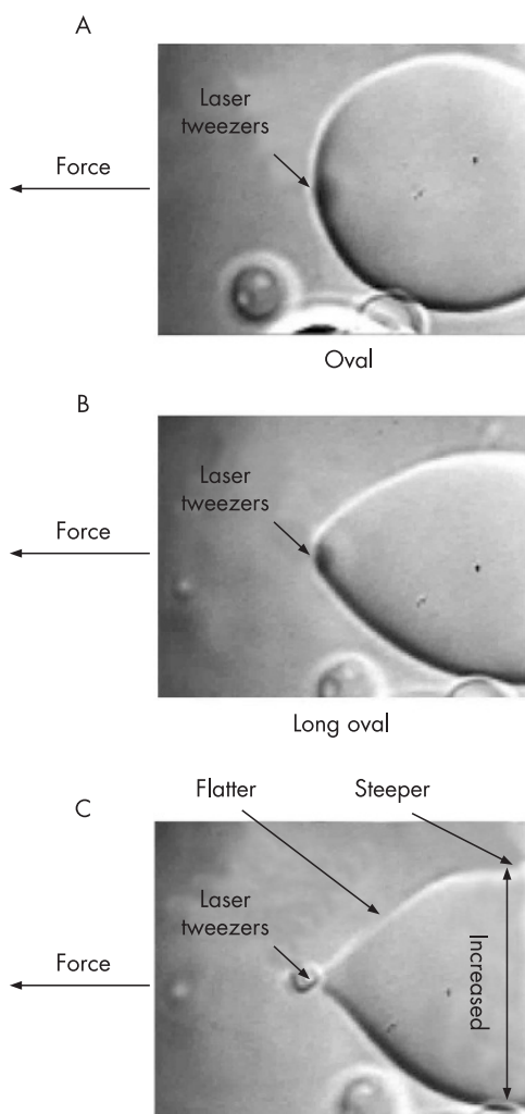
Figure 6 Vesicle profiles during application of an outwardly increasing equatorial force applied externally by optical tweezers. (A) Demonstrates an oval profile. (B) Demonstrates further elongation of the vesicle in the axis of force resulting in a long oval profile. (C) Demonstrates the central steepening, peripheral flattening, and increased central thickness associated with a small increase in the equatorial diameter of the long oval profile.
