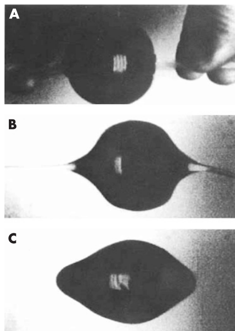
Figure 7 Changes in shape of a freely floating 6 cubic inch drop of water in the microgravity environment of the SKYLAB in response to manual application of equatorial traction. (A) Demonstrates the baseline circular water drop profile. (B) Demonstrates elongation of the water drop profile in the axis of force. (C) Demonstrates central steepening and peripheral flattening of the water drop profile (reproduced with permission from the National Aeronautics and Space Administration, NASA).
