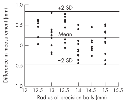
Figure 3 A Bland-Altman plot 21 of the difference between the measured radius and the actual radius of the precision balls.
