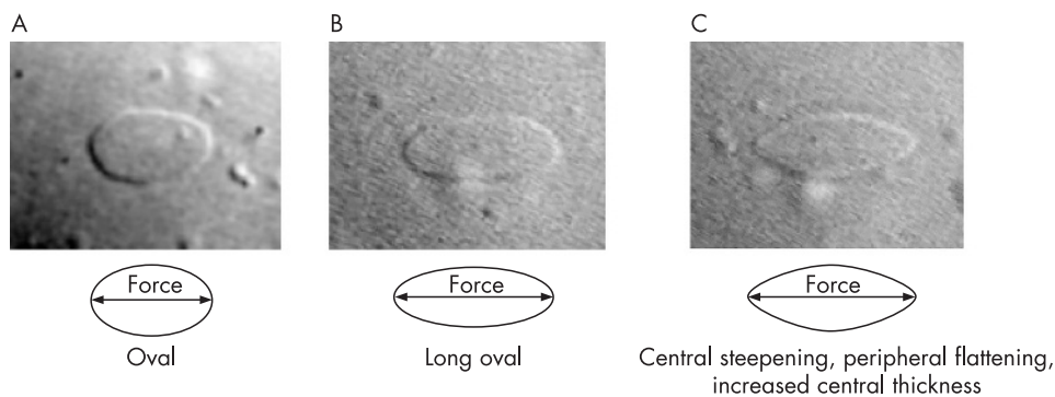
Figure 5 Vesicle profiles during an outwardly increasing equatorial force applied from within the vesicles by microtubule polymerisation. (A) Demonstrates an oval profile. (B) Demonstrates further elongation of the vesicle in the axis of force resulting in a long oval profile. (C) Demonstrates the central steepening, peripheral flattening, and increase in central thickness associated with a small increase in the equatorial diameter of the long oval profile.
